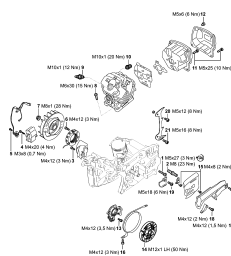
Tightening torques
