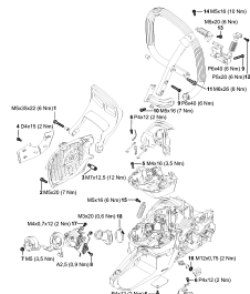
Tightening torques
