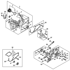
Crankcase
