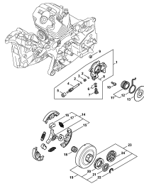
Oil pump, Clutch
