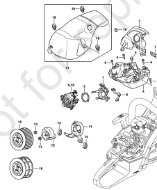
Carburetor bracket, Air filter, Shroud M-Tronic
