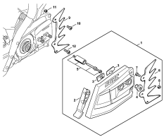
Chain sprocket cover
