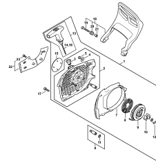
Rewind starter M-Tronic
