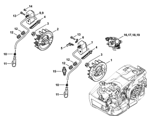
Ignition system
