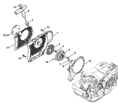
Rewind starter
