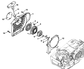
Rewind starter ErgoStart/Easy2Start
