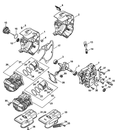
Crankcase, Cylinder, Muffler
