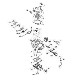
Carburetor C1Q-S251, C1Q- S249, C1Q-S215, C1Q- S189
