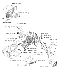
Tightening torques
