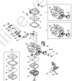
Carburetor 1145/22, 1145/27, C1Q-S274
