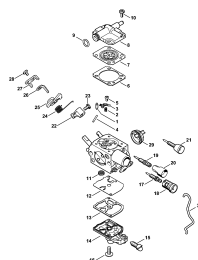
Carburetor C1Q-S281, C1Q- S284
