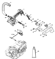
Handle housing, Handlebar M-Tronic
