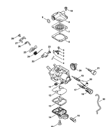
Carburetor C1Q-S280, C1Q- S283
