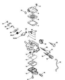
Carburetor C1Q-S250, C1Q- S248, C1Q-S214, C1Q- S188
