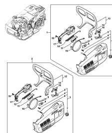
Chain sprocket cover, Hand guard
