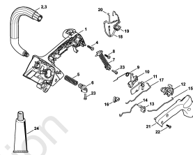
Handle housing, Handlebar
