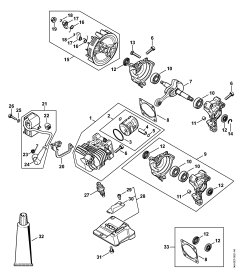
Cylinder with piston, Ignition system
