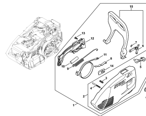
Chain sprocket cover
