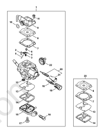
Carburetor 1146/05
