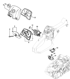
Air filter, Carburetor box cover
