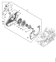
Rewind starter
