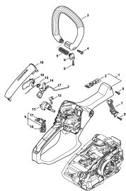
Handle housing, Handlebar
