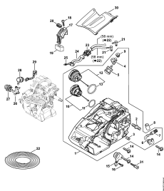
Motor housing
