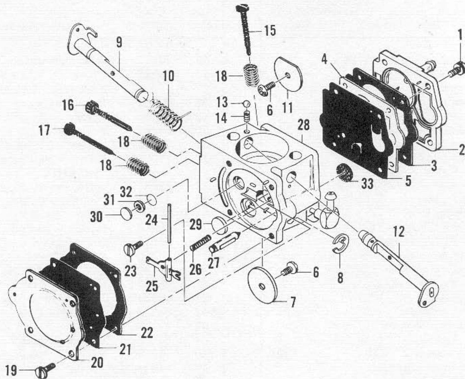
Figure 5. Carburetor Assembly
