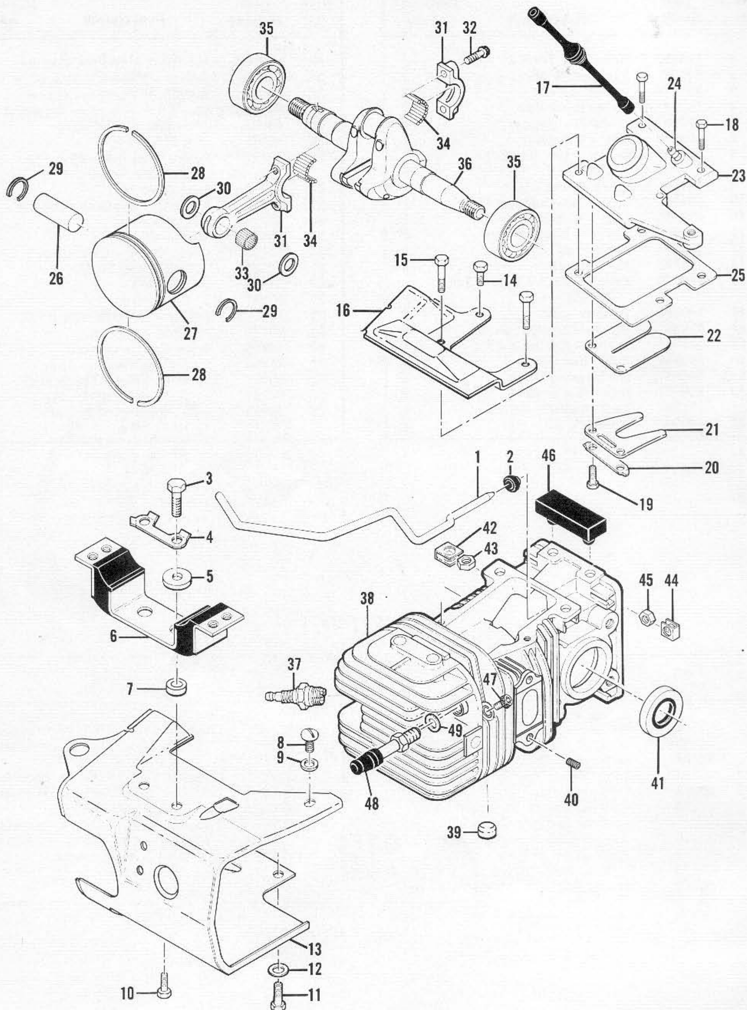
Figure 8. Powerhead & Shroud Assemblies
