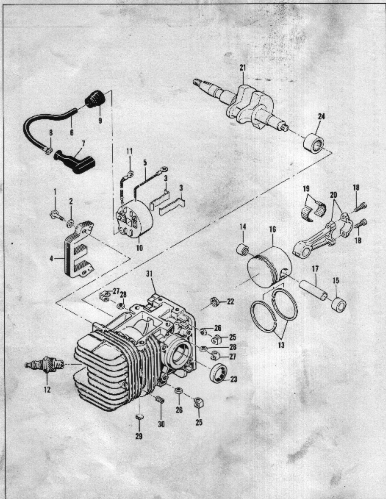
Figure 6. Powerhead
