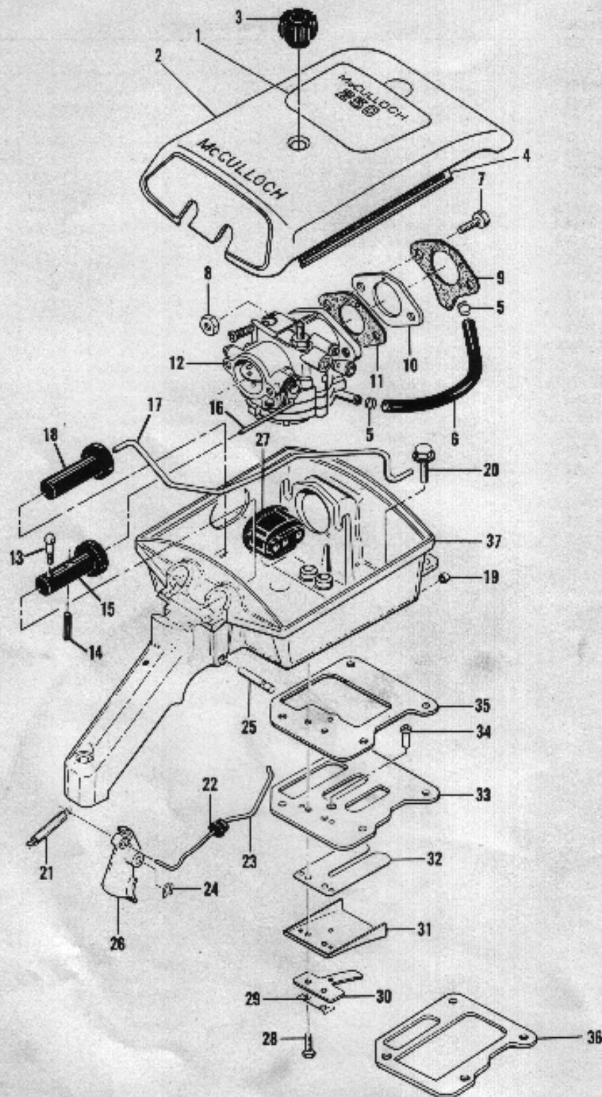
Figure 4. Cover and Airbox Assemblies
