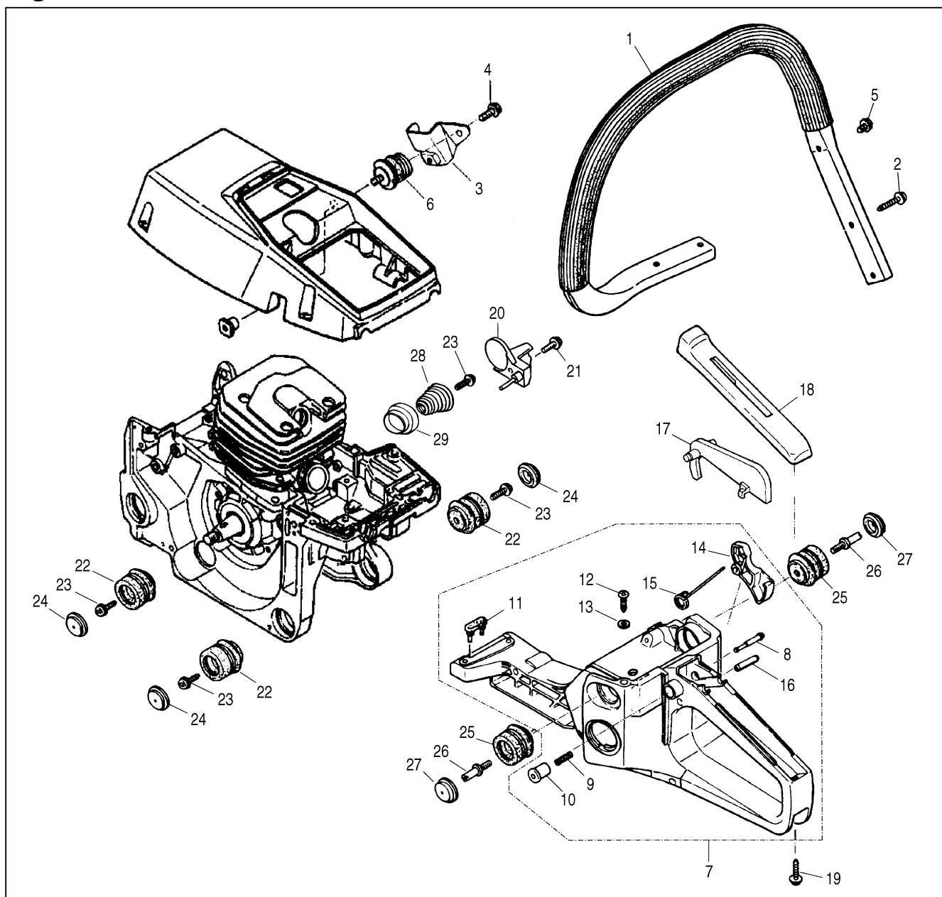
Fig.3 HANDLES
